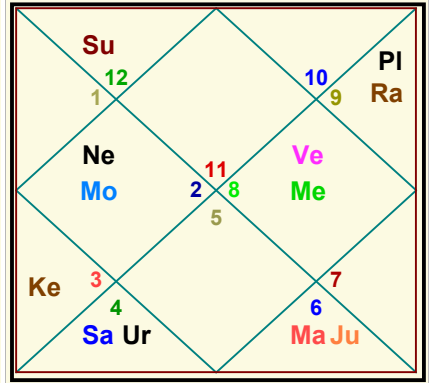
Navamsha Chart
