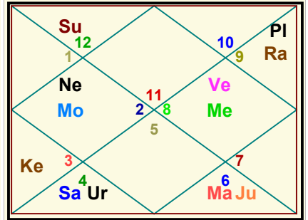
Navamsha Chart
